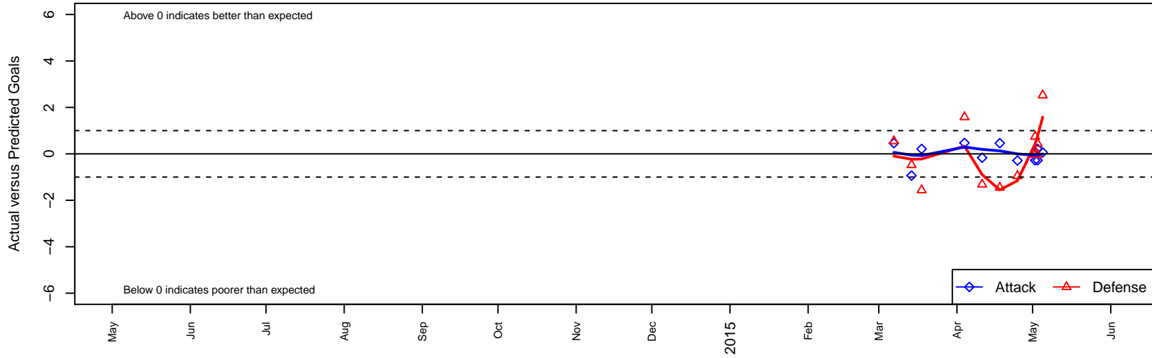
Idaho Rush Nero G99 Dots are actual minus expected GF (blue circles) and GA (red triangles). Blue line is smoothed change in attack strength. Red is smoothed change in defense strength.
